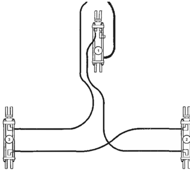
3 Cylinder System with One Master
