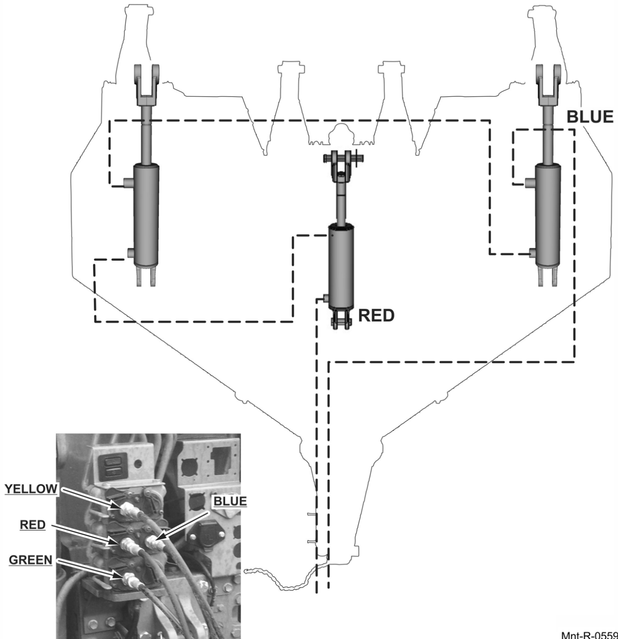
AXLE CYLINDER HYDRAULIC SCHEMATIC
